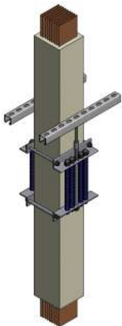
Open Spring Support in Hanging Arrangement
