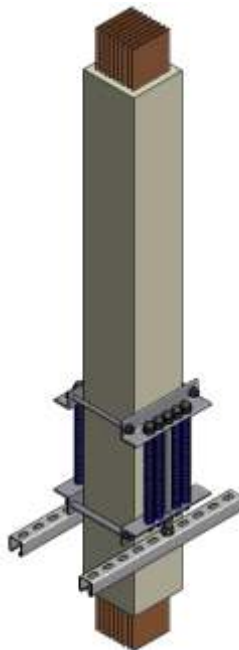
Open Spring Support in Standing Arrangement
